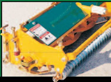
Floating mower head with front grooved roller for low mowing heights.
